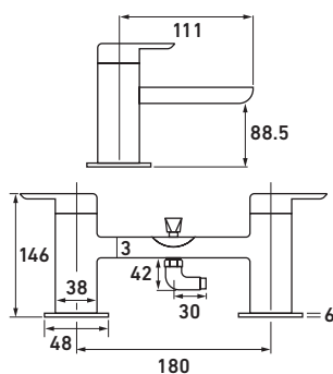
BATH SHOWER MIXER with kit, deck mounted VOS330K1
