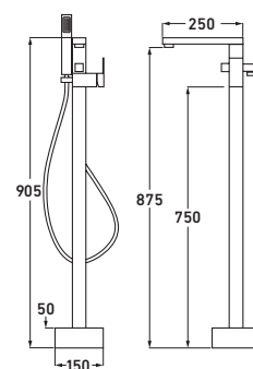
FLOOR STANDING BATH SHOWER MIXER with kit VOSFS301
