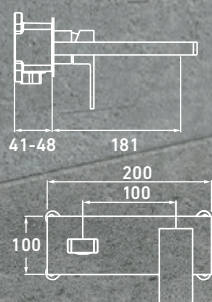
WALL MOUNTED BASIN MIXER VOS441 £186.52
